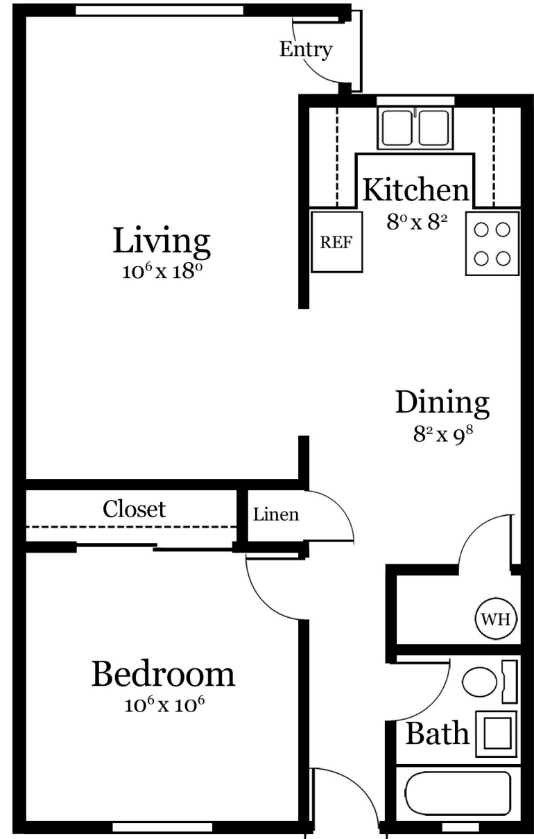
Inside Unit
